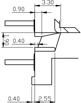
SEC B (3:1)
