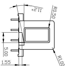
SEE F-F
