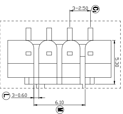
DETAIL I SCALE 2:1
