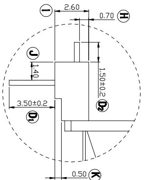
DETAIL I SCALE 2:1
