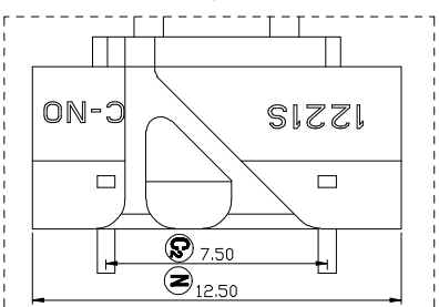
DETAIL H SCALE 2:1
